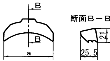
爪 (FCD450-10)
