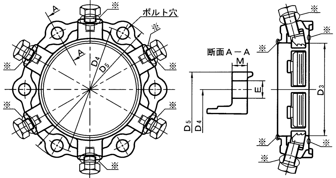
爪 (FCD450-10)
