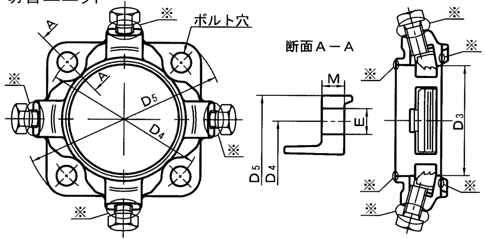
爪 (FCD450-10)
